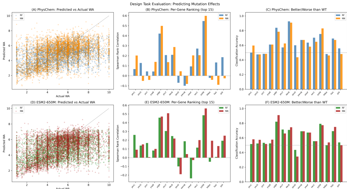
Figure 6: Design task evaluation. Model predictions for 4832 designed signal peptide variants across 131 genes (requiring \geq 5 variants per gene), comparing physicochemical features (top row) and ESM2-650M embeddings (bottom row) with both RF and NN models.
