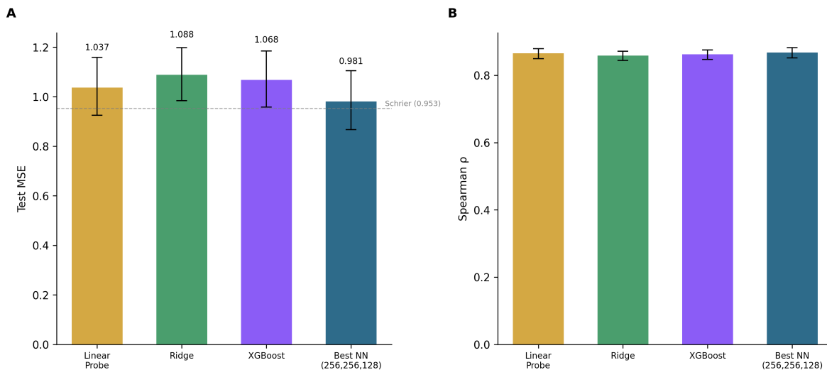
Figure 7: Baseline comparison. (A) Test MSE with 95% bootstrap CIs. (B) Spearman \rho with 95% bootstrap CIs. The linear probe (no hidden layers) captures most of the embedding’s predictive power; the MLP provides a modest additional improvement.
