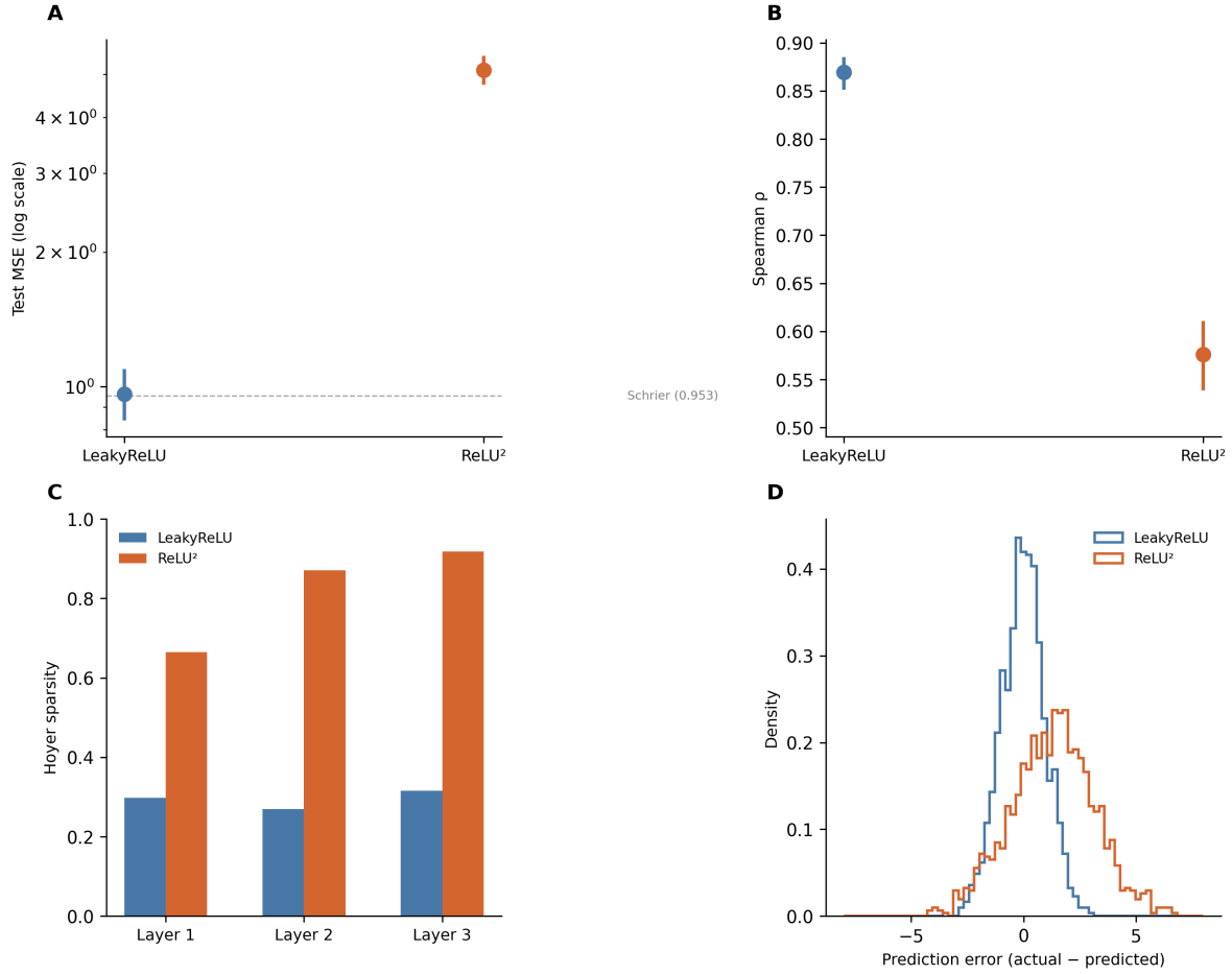
Figure 16: ReLU-squared vs LeakyReLU activation comparison. Despite producing sparser hidden representations (Hoyer sparsity 0.67–0.92 vs 0.27–0.32), ReLU-squared degrades prediction accuracy from MSE 0.961 to 5.11.
