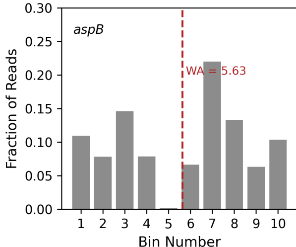
Figure 1: Bimodal bin probability distribution for gene aspB , variant MKLAKRVSALTP-STTLAITQKAKEL (WA = 5.63). The weighted average (dashed line) falls in the valley between peaks at bins 3 and 7, illustrating that the scalar WA can be a poor summary of the underlying distribution.
