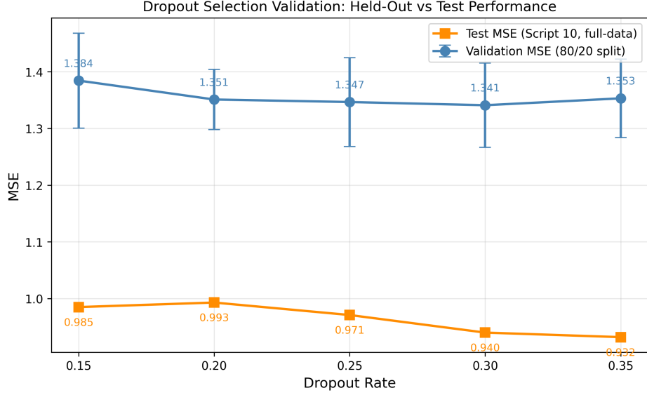
Figure 10: Dropout validation: MSE on held-out validation data (80/20 split, blue) versus test data (full-data training from Script 10, orange). Both curves show the same general trend: increasing dropout from the base rate of 0.20 improves performance. Error bars on validation MSE represent standard deviation across 5 seeds. Absolute validation MSE is higher because models train on only 80% of the data.
