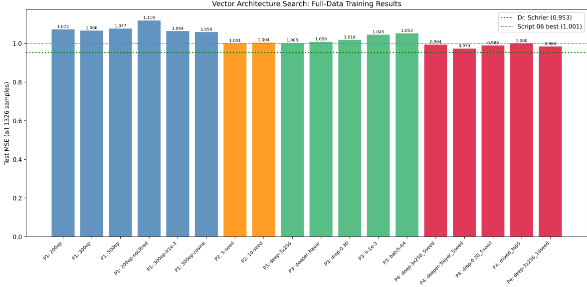
Figure 8: Architecture search results for full-data vector regression (Ginkgo-AA0 + focal loss). Configurations are ranked by test MSE on all 1326 test samples. The three-layer (256, 256, 128) architecture with 5-seed ensemble achieved the lowest MSE (0.973), motivating the subsequent dropout optimization (Section 3.4).
