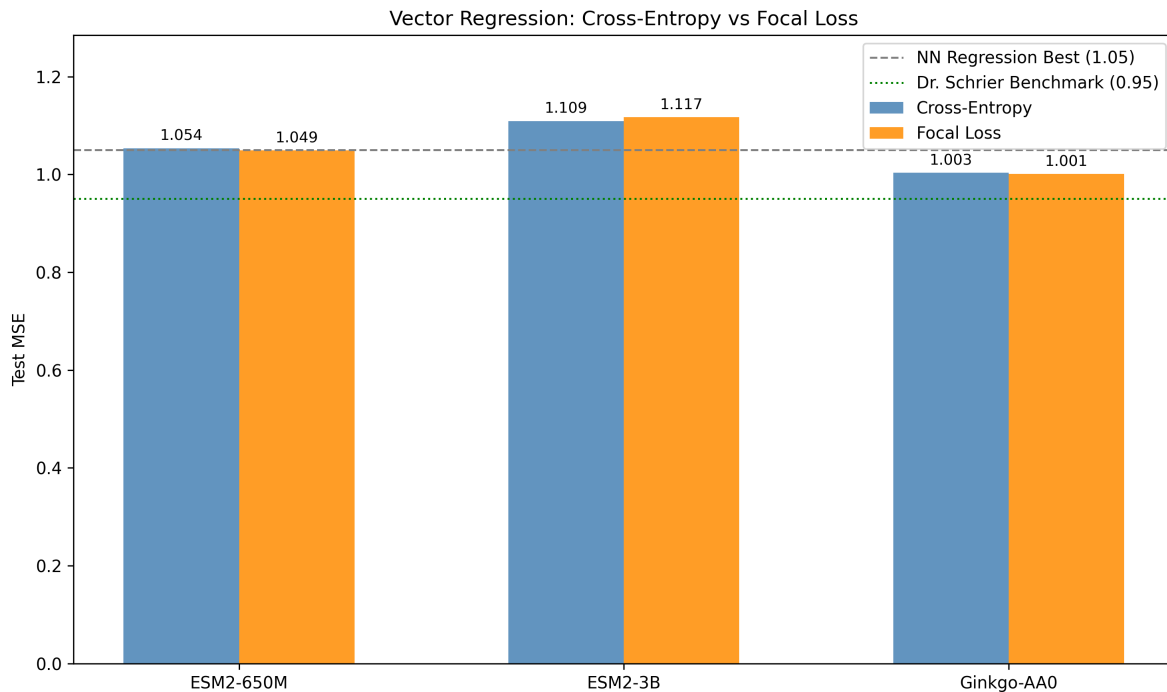
Figure 4: Vector regression results comparing three PLM embedding types and two loss functions. Ensemble MSE values are annotated above each bar.
