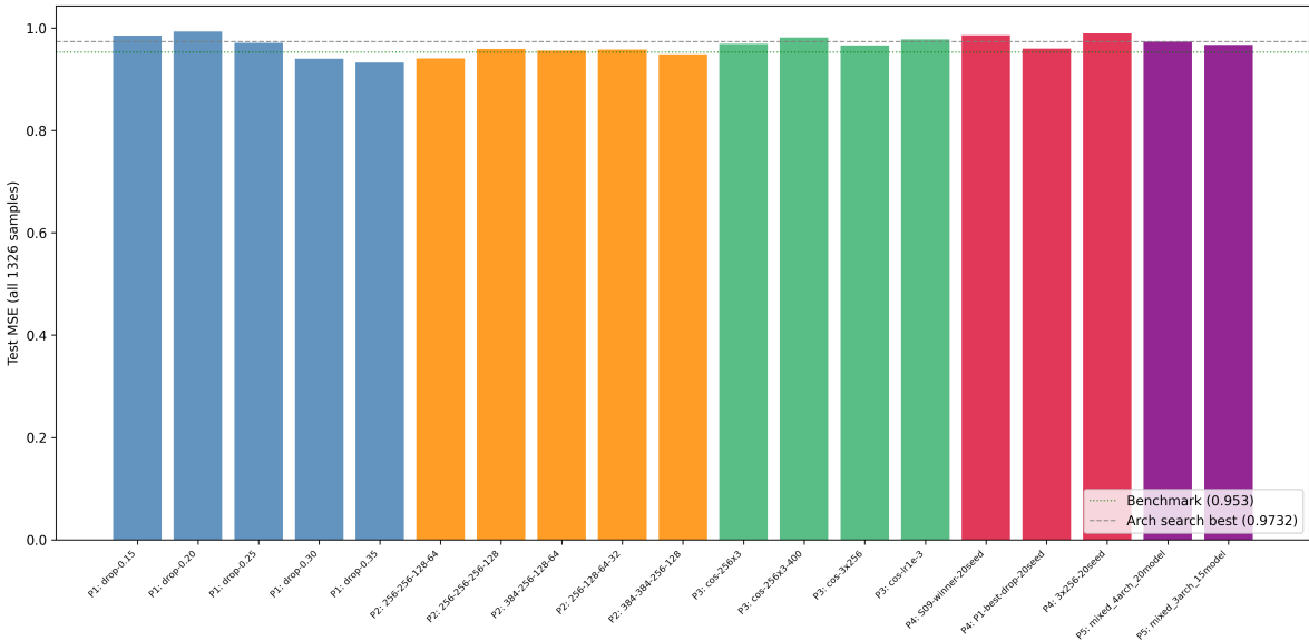
Figure 5: Full-data vector regression optimization results. Configurations are grouped by optimization phase; the dotted green line indicates an unpublished single-model result of 0.953 for comparison; the dashed grey line shows the initial architecture search best (0.973).
