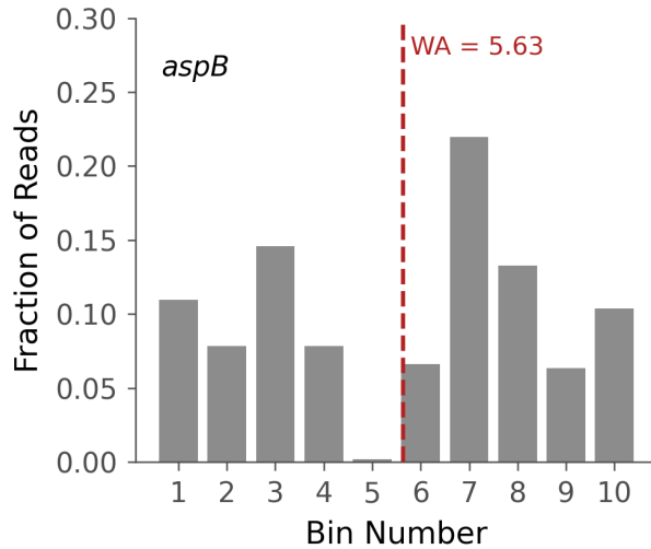
Figure 1: Bimodal bin probability distribution for gene aspB , variant MKLAKRVSALTP-STTLAITQKAKEL (WA = 5.63). The weighted average (dashed line) falls in the valley between peaks at bins 3 and 7, illustrating that the scalar WA can be a poor summary of the underlying distribution and motivating the vector regression approach.
