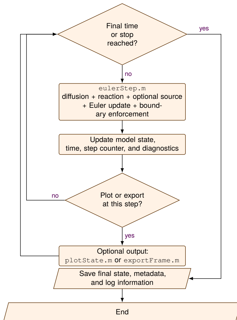
Figure 6.2.: Repeated simulation loop of the final Gray–Scott solver.
