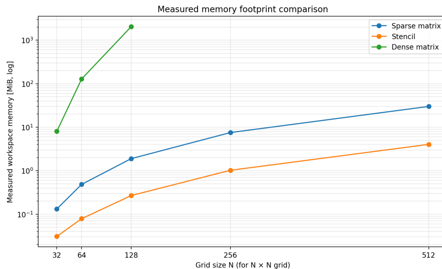
Figure 10.4.: Measured memory footprint of the solver realizations. The y-axis is shown in MiB on a logarithmic scale.
