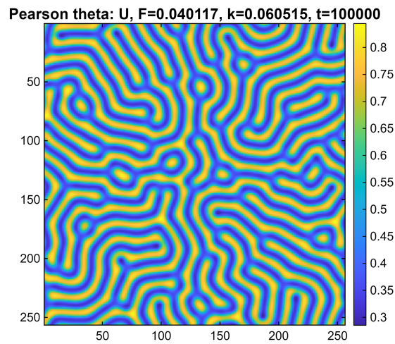
Figure 8.10.: Pearson \theta case: representative U -field snapshot at t = 100000 . The pattern is also labyrinth-like, but with a more intricate and locally curved stripe network than in the \kappa case.
