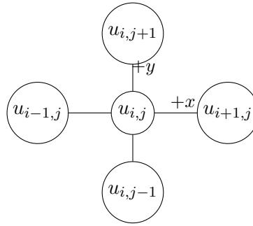
Figure 4.1.: Five-point finite-difference stencil used for the discrete Laplacian on the two-dimensional Cartesian grid.
