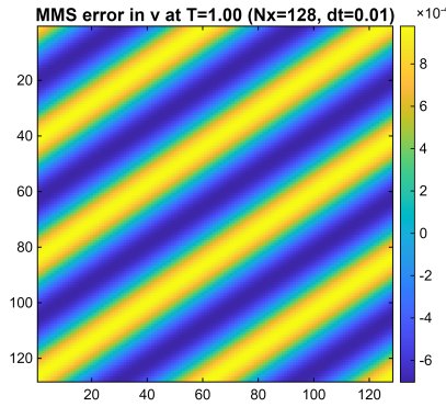
Figure 8.6.: Spatial error field of the manufactured-solution end-to-end test for v at T = 1 , with N_x = N_y = 128 and \Delta t = 0.01 .
