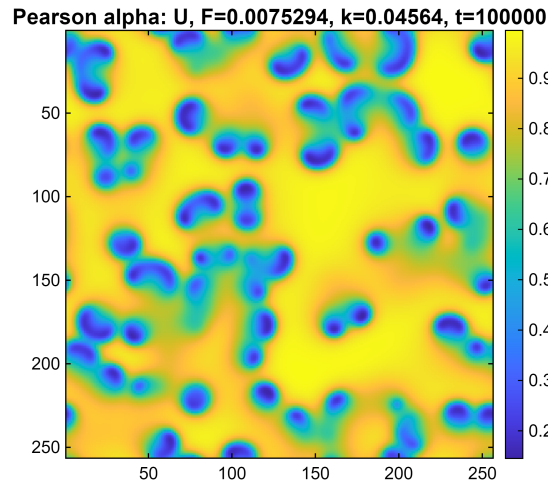
Figure 8.7.: Pearson alpha case: representative U -field snapshot at t = 100000 . The morphology is dominated by separated spot-like structures in a mostly high- U background.
