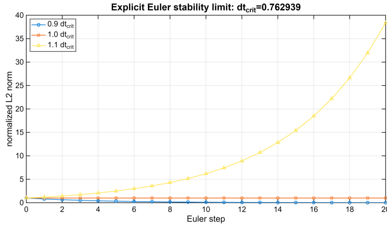
Figure 8.5.: Explicit Euler stability-limit test for the diffusion subcase on the 128 \times 128 periodic grid. Below the critical time step the perturbation decays, at the critical value it is preserved, and above the critical value it grows, in exact agreement with the theoretical amplification factors.
