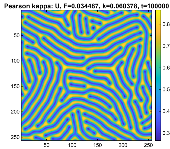
Figure 8.9.: Pearson kappa case: representative U -field snapshot at t = 100000 . The pattern exhibits a broad labyrinth-like stripe morphology rather than isolated spots.
