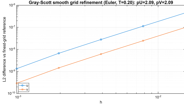
Figure 8.4.: Final Gray–Scott grid-refinement study using the 2048 \times 2048 solution as a numerical reference and a smooth grid-independent initial condition. The measured L^2 differences in U and V decrease monotonically and yield observed rates p_U = p_V \approx 2.09 , consistent with second-order spatial behavior.
