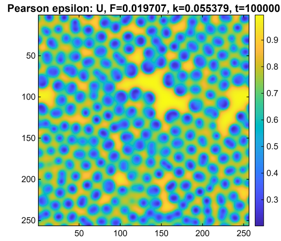
Figure 8.8.: Pearson epsilon case: representative U -field snapshot at t = 100000 . Compared with alpha , the pattern is denser and more uniformly populated by small spot-like structures.
