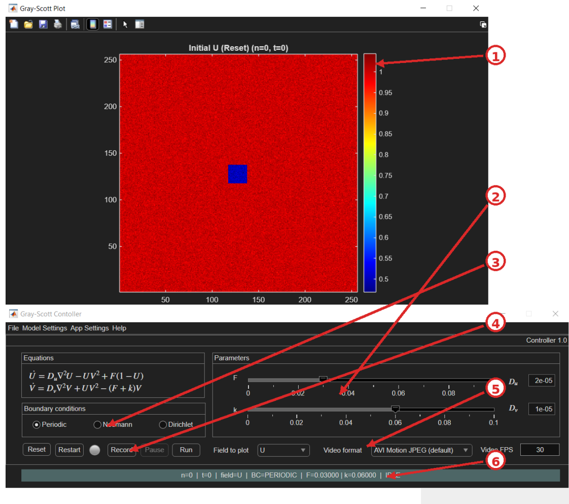
Figure A.1.: Annotated screenshot of the final GUI during a typical startup state. The numbered callouts indicate the main elements used during interactive operation.
