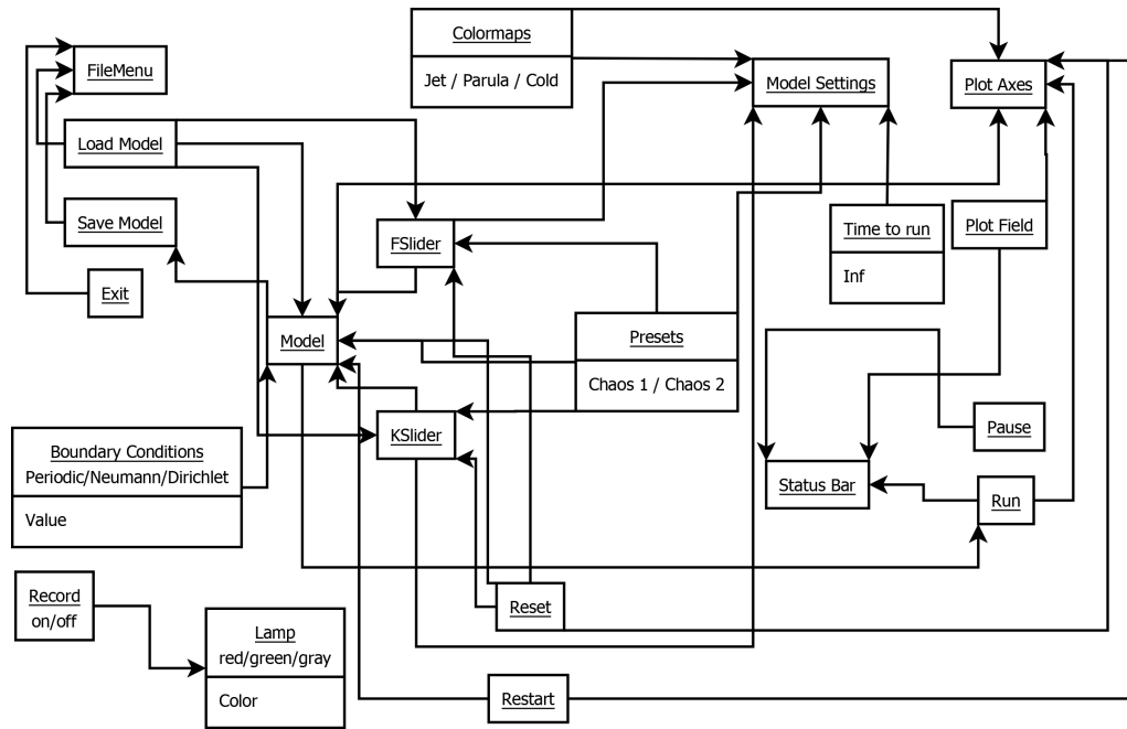
Figure 4.6.: Information flow between the main GUI elements, the shared model state, and the visualization components.
