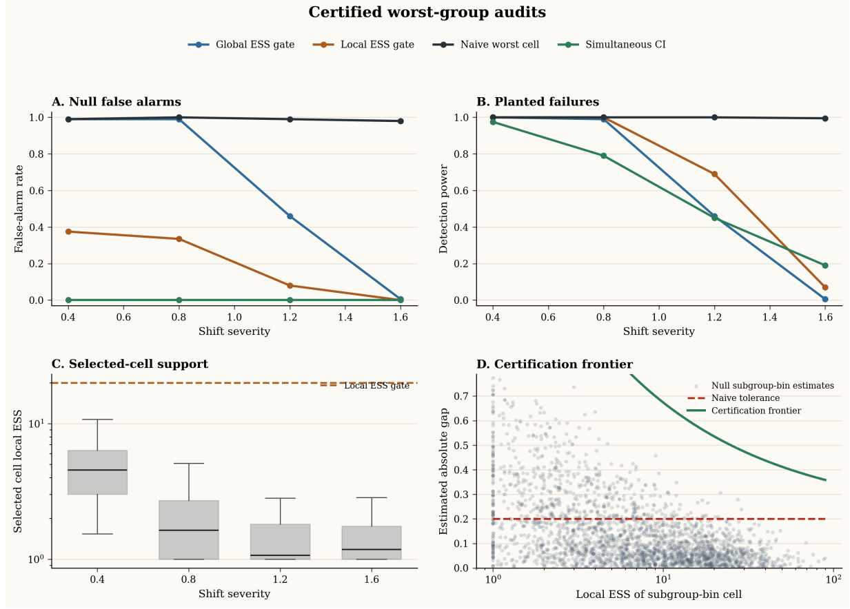
Figure 1: Synthetic covariate-shift audit. Point-estimate and global-ESS rules false-alarm under the null; simultaneous local certificates control false alarms and lose power as local overlap weakens.
