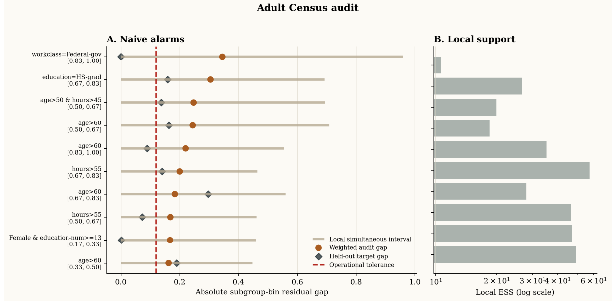
Figure 3: Adult Census audit. The largest naive alarms have wide local intervals and small held-out target gaps; certification reports insufficient evidence.
