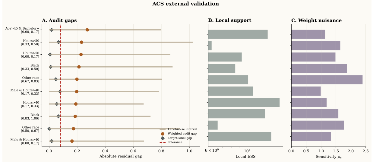
Figure 4: ACSIncome external validation. Large naive gaps coexist with low local ESS and learned-weight sensitivity; held-out target labels support the insufficient-evidence decision.
