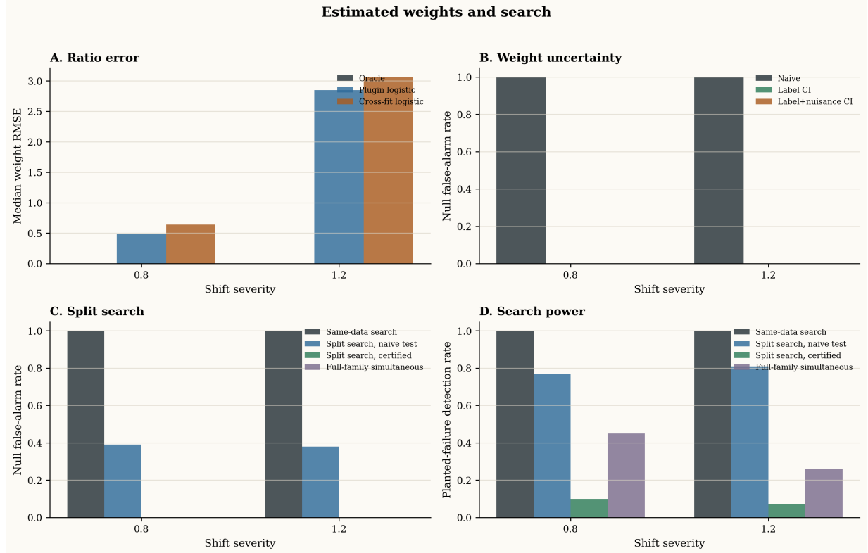
Figure 2: Estimated weights and adaptive search. Ratio estimation and subgroup search add uncertainty beyond the oracle local-ESS setting.
