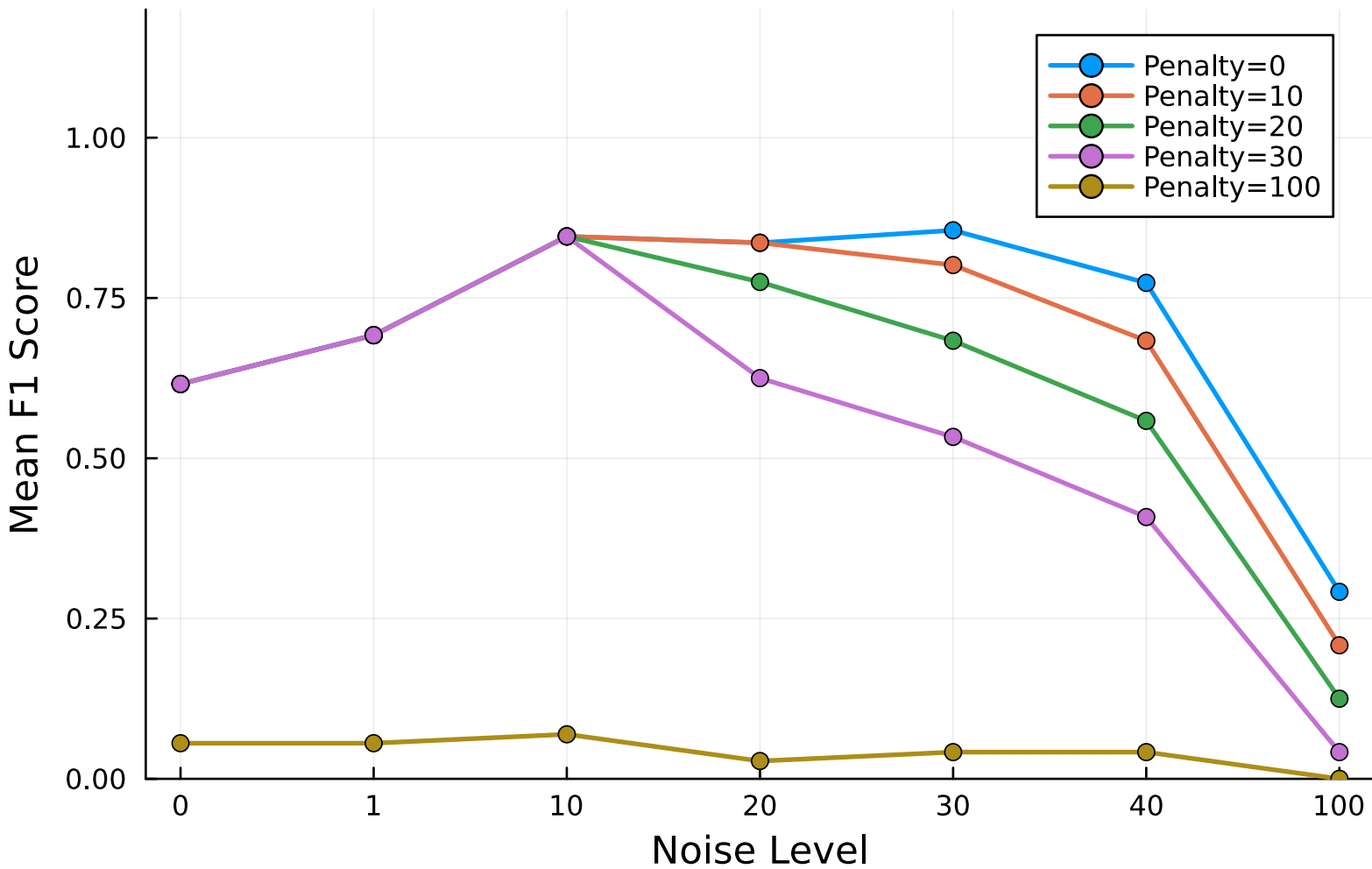
Effect of BIC Penalty Coefficients on F1 Score Across Noise Levels
