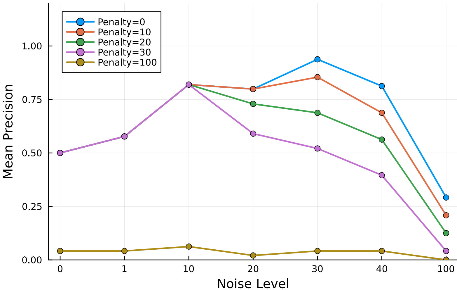
Effect of BIC Penalty Coefficients on Precision Across Noise Levels
