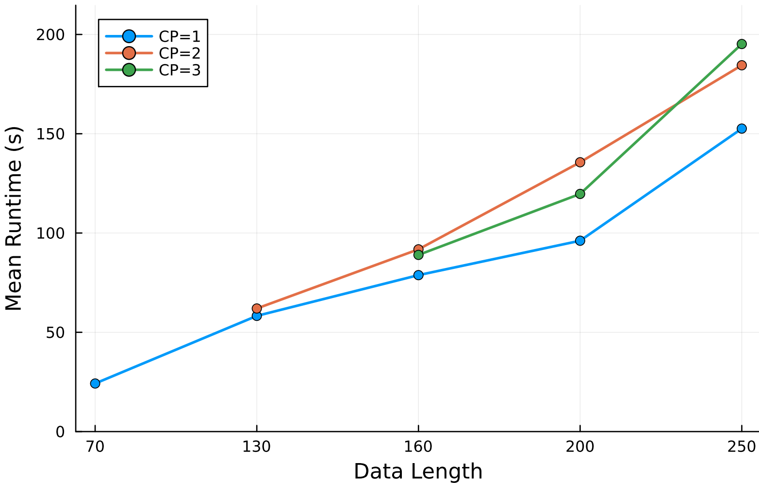
Runtime vs Data Length for Different Change Point Counts
