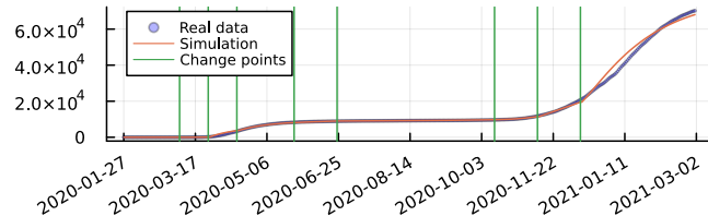
Death
