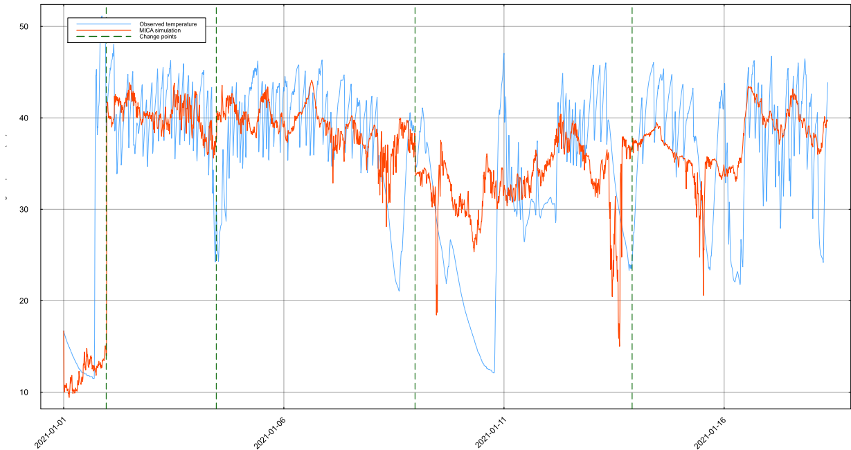
Fig 13. Wind-turbine generator front-bearing temperature fitted with MICA using BIC/MDL/AIC model selection. Observed temperature (blue), MICA simulation (orange), and the four detected change points (green dashed vertical lines). The BIC, MDL, and AIC criteria all returned the same four change points.
