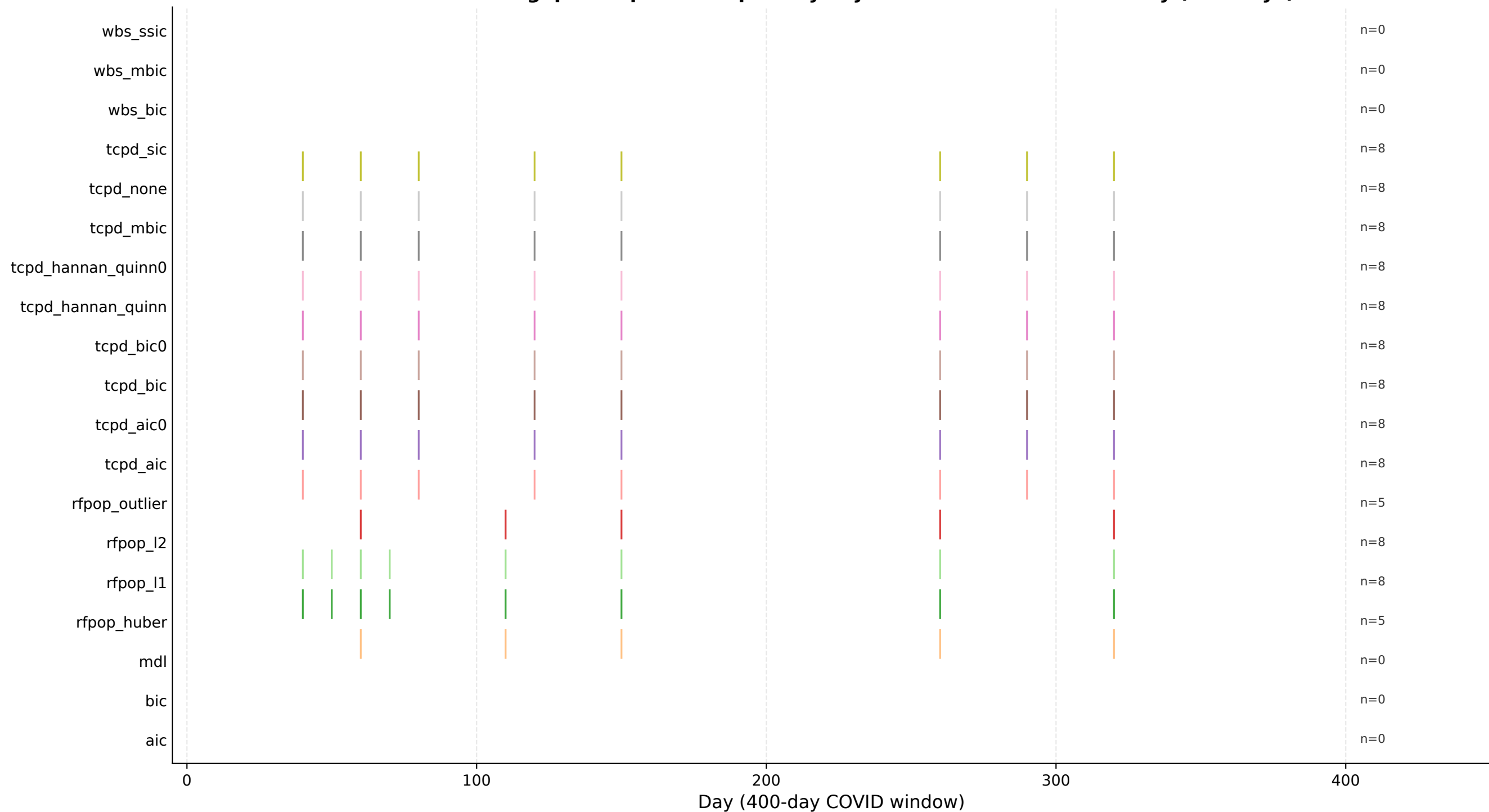
Detected changepoints per TCPD penalty objective — COVID-19 Germany (400 days)
