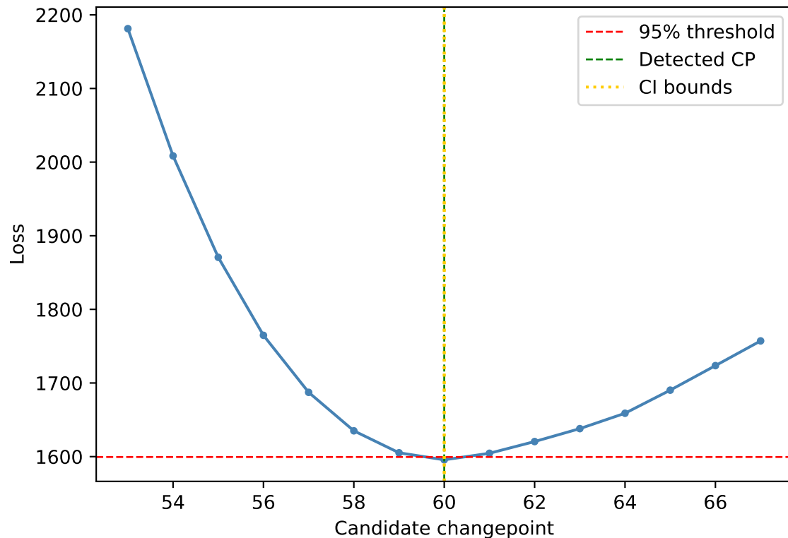
CP 1 (original=60) CI = [60, 60], identifiable=True
