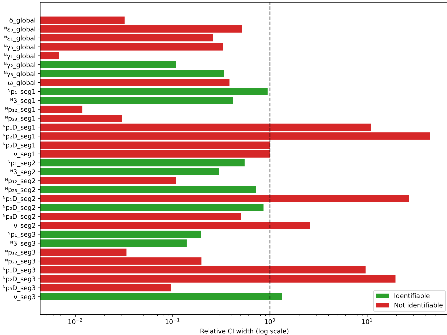
COVID conditional PLE: parameter identifiability (L1 CPD + L2 PLE, 2 CPs [60,150])
