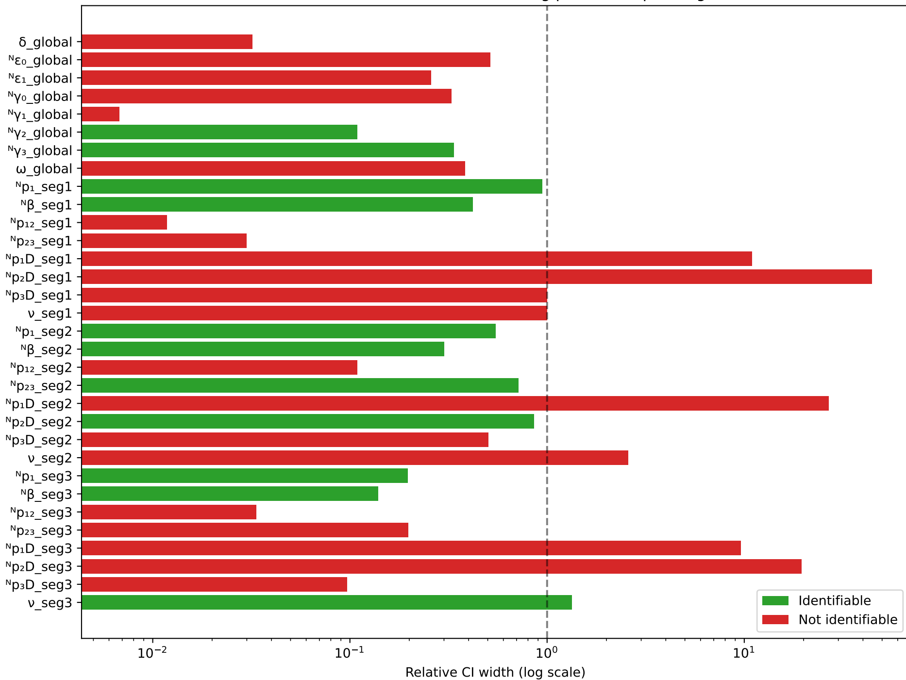
COVID 'joint' PLE: parameter identifiability (L1 CPD + L2 PLE, CPs fixed during parameter profiling)
