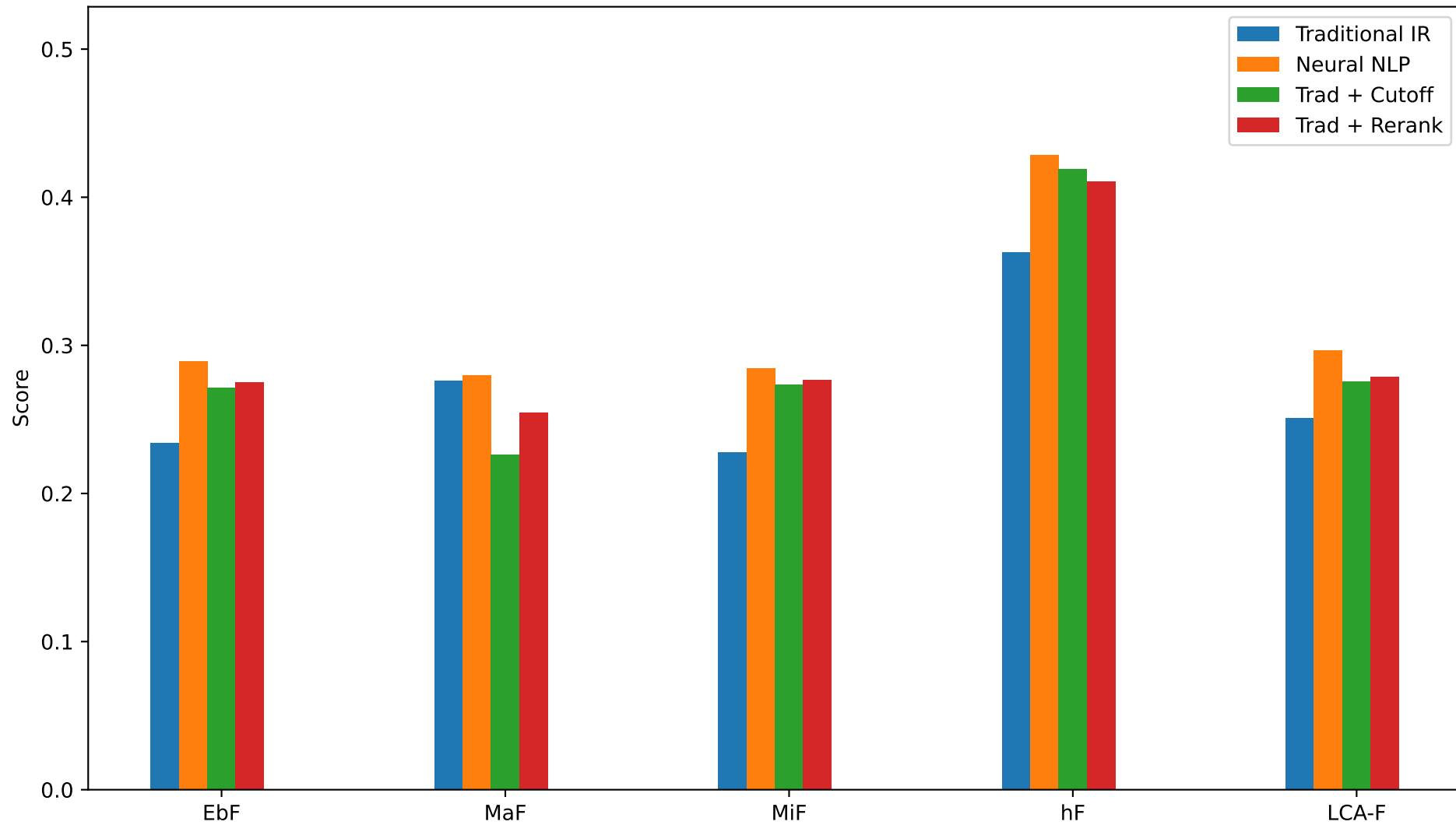
Models compared by F scores
