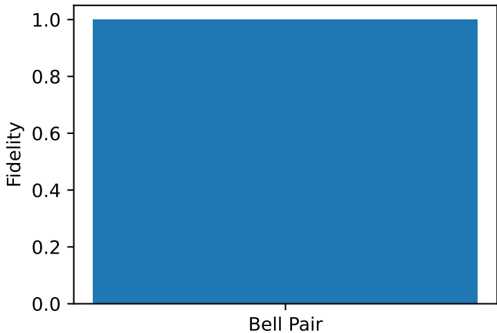
Bell Pair Fidelity
