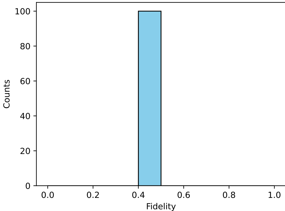
Quantum Switch Fidelity (3 clients)
