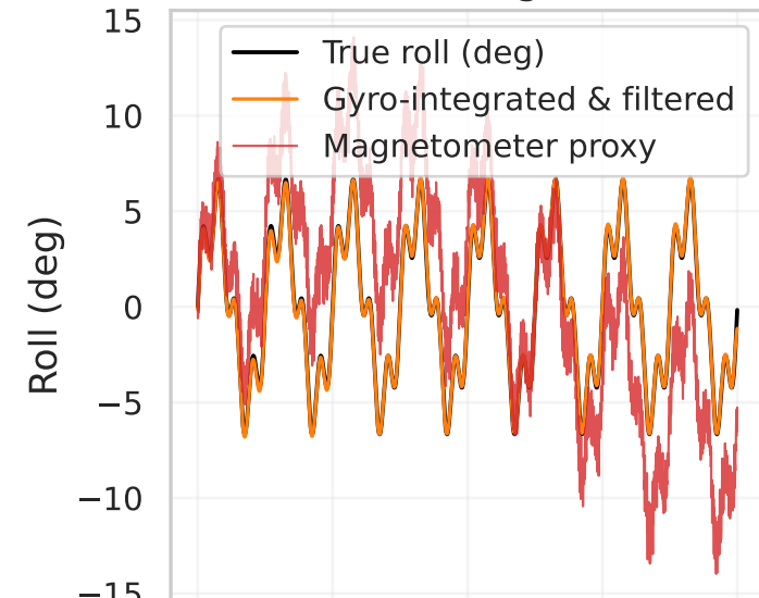
Roll &amp; Alt — magnetic bias
