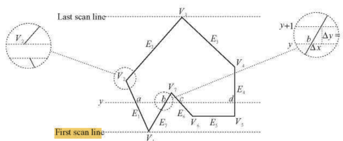
Fig. 3-19 Scan-converting a polygonal region.
