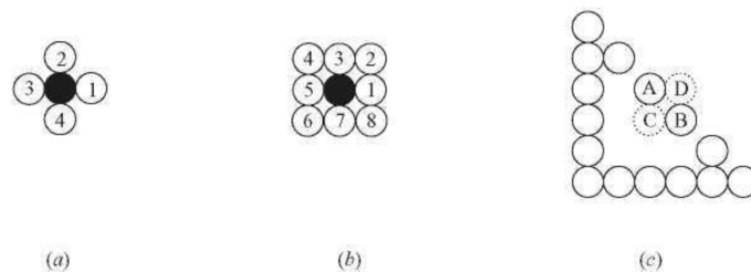
Fig. 3-18 4-connected vs. 8-connected pixels.
