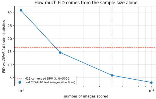
Figure 9: FID of real CIFAR-10 test images against sample size, three draws per size. The dashed line is our converged DPM-Solver-3 at 5,000 samples. Real images follow FID \approx 3.0 \times 10^4/N , which sets a floor of 5.9 at our sample size.
