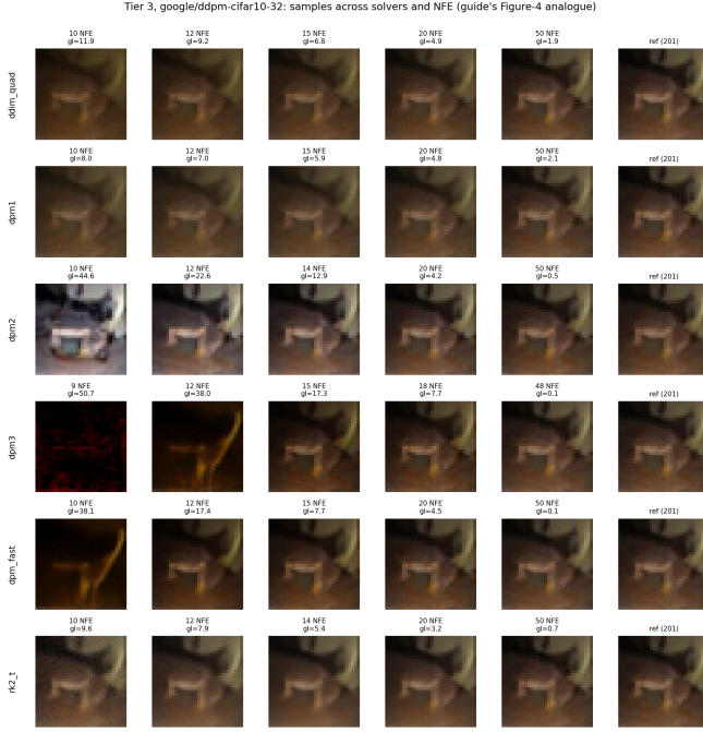
Figure 8: One starting noise, six samplers, five budgets, and the 201-NFE reference (right). “gl” is the mean absolute difference from the reference in 8-bit gray levels. At 10 NFE, DDIM and DPM-Solver-1 give the right picture, blurred; DPM-Solver-2 gives a sharp but different picture; DPM-Solver-3 at 9 NFE gives noise. By 20 NFE all samplers are visually close to the reference.
