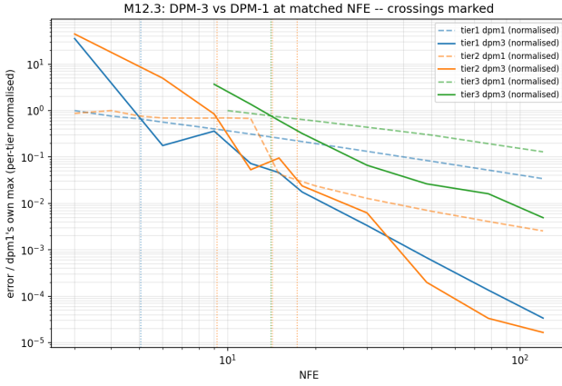
Figure 6: DPM-Solver-3 (solid) against DPM-Solver-1 (dashed) at matched NFE, each tier normalised by its own DPM-Solver-1 maximum. Dotted verticals mark crossings.
