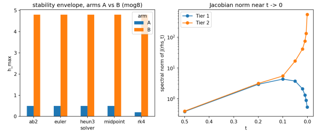
Figure 7: Stability on Tier 2. Left: largest stable step per step; bars at 0.4995 (in t ) and 4.79 (in \lambda ) are the coarsest grids tried, so those steppers never diverged, and only arm-A RK4 is limited. Right: spectral norm of the arm-A Jacobian along the trajectory; Tier 1 turns down near t \rightarrow 0 while Tier 2 climbs to 545.
