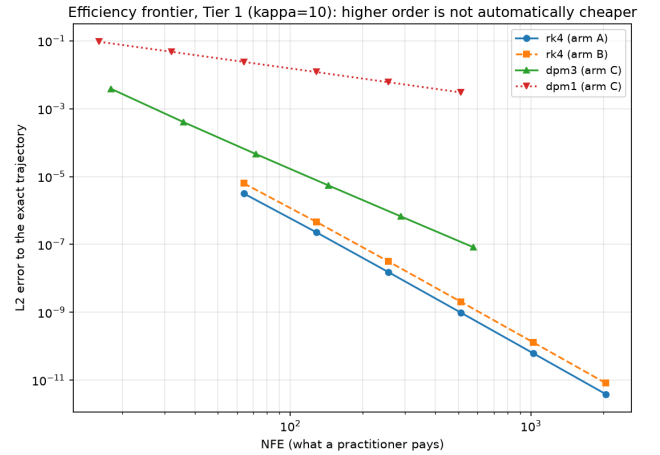
Figure 5: Tier 1 ( \kappa = 10 ), asymptotic protocol: error against measured NFE, the cost a user pays. RK4 in either variable stays below DPM-Solver-3 at every shared budget.
