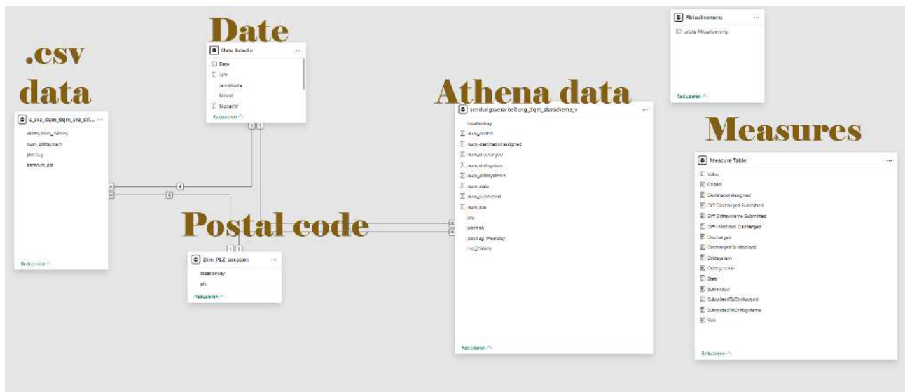
Figure 5.4.: Initial Power BI data model containing the core tables required for the first report prototype
