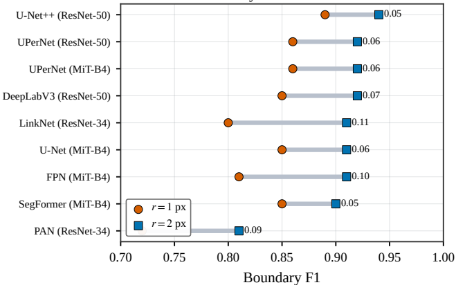
BF1 Sensitivity to the Tolerance Radius
