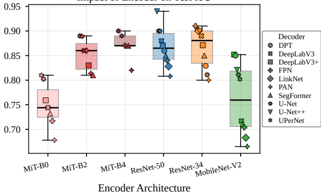
Impact of Encoder on Test IoU
