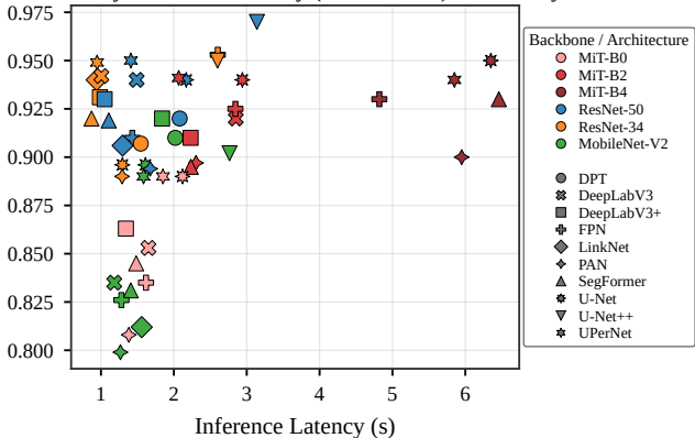
Efficiency Frontier: Accuracy (Test Dice F1) vs. Latency
