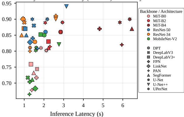
Efficiency Frontier: Accuracy (Test IoU) vs. Latency
