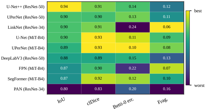
Topology-Aware Evaluation Matrix (Test Set)
