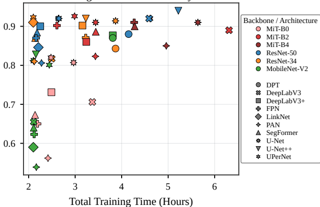
Training Cost vs Test Boundary F1
