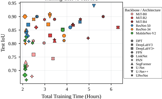
Training Cost vs Test IoU
