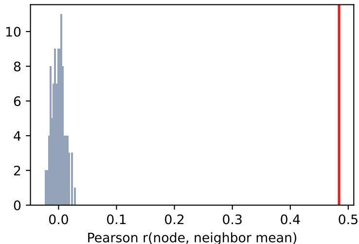
PBE, \phi=0.9 ( z=43.9 )
