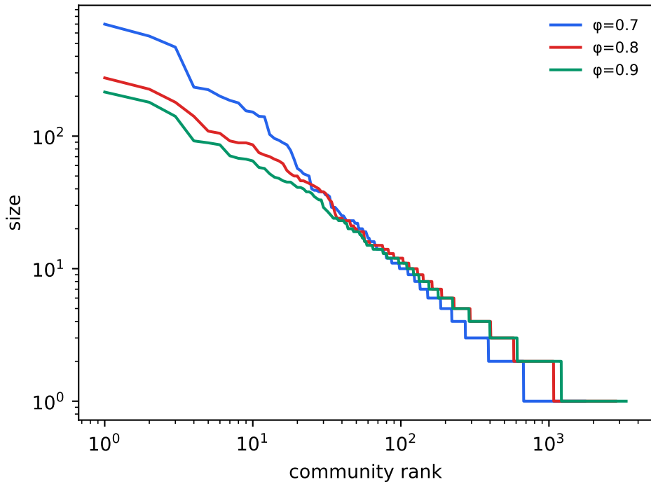
Leiden community sizes
