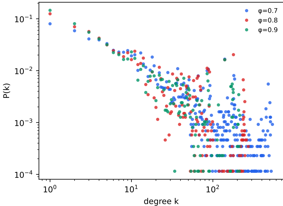
Degree distribution (isolated nodes omitted)
