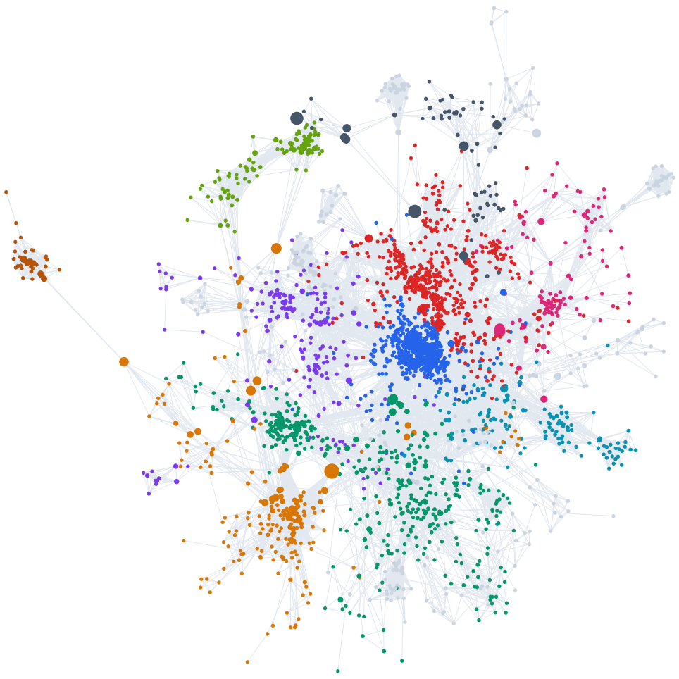
Giant component (3000 of 3659 nodes shown); colour = Leiden community (10 largest), size = betweenness
