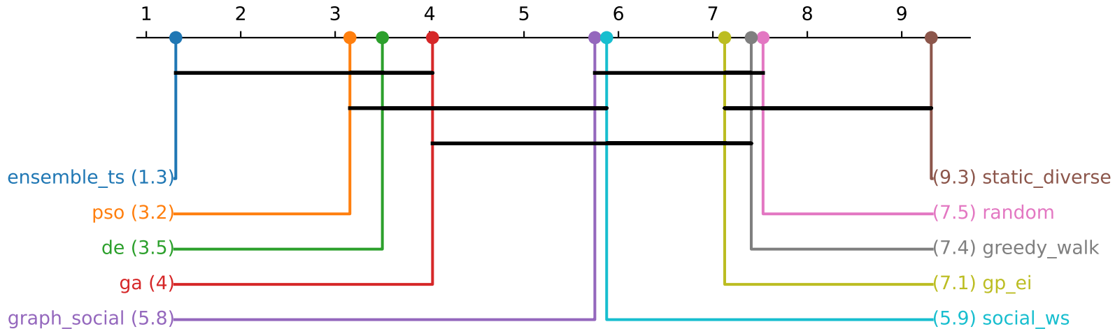
Mean rank across objective \times budget blocks (final recall; 1 = best)
