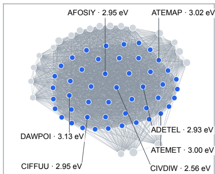
c Building-block near-clique: \text{Zn} | \text{C}_8\text{H}_4\text{O}_4^{2-}
