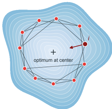
a SOCIAL (previous work) continuous search space, synthetic small-world agent graph
