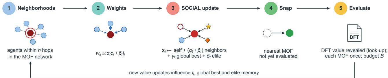
c One Graph-SOCIAL iteration (SOCIAL learning rules unchanged)
