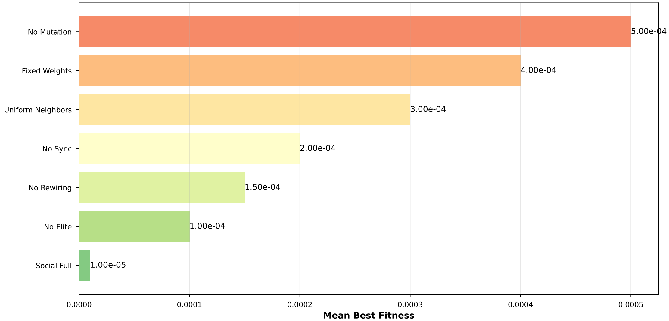
Ablation Study: Mean Best Fitness by Variant
