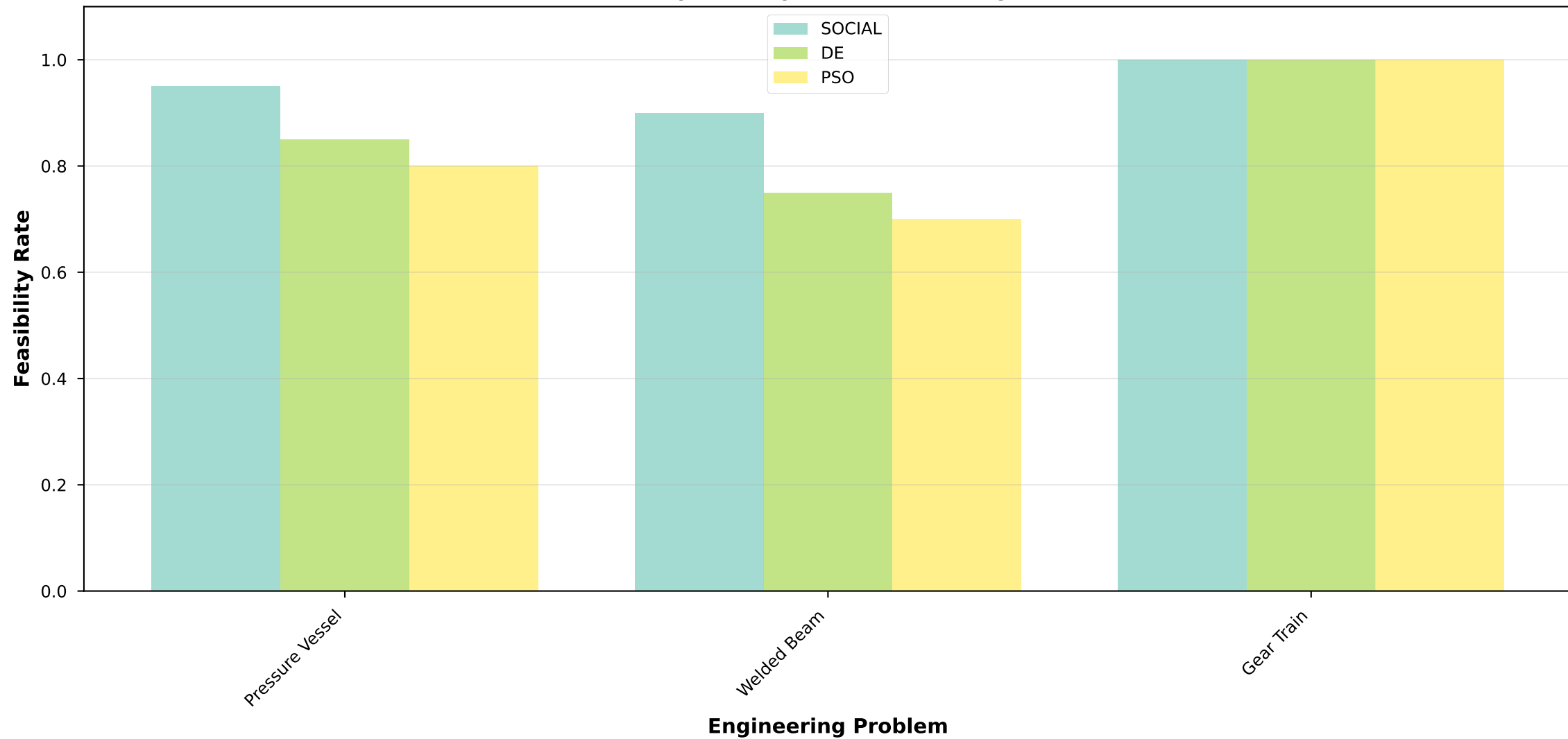
Feasibility Rate by Problem and Algorithm
