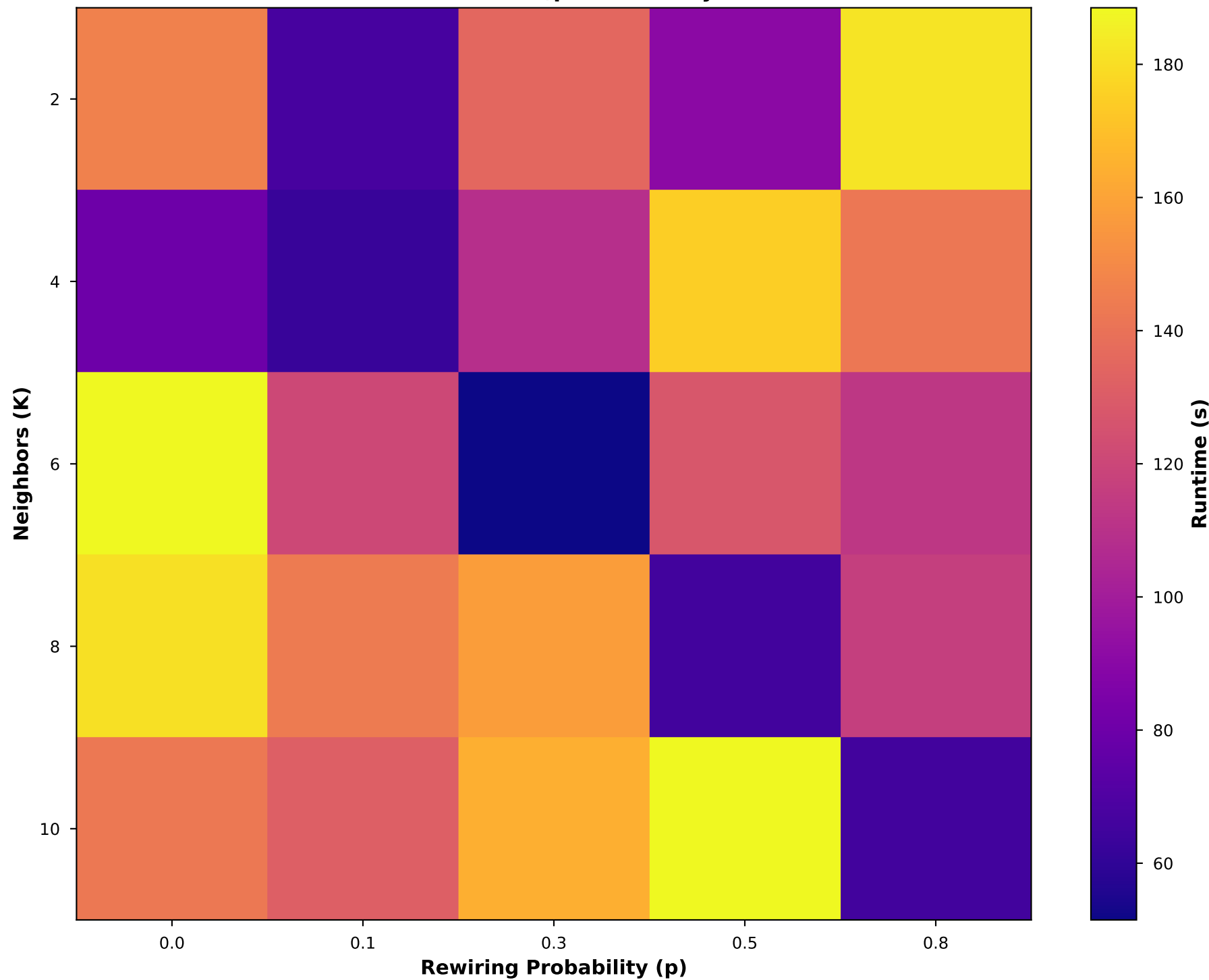
Runtime - (K,p) Sensitivity
