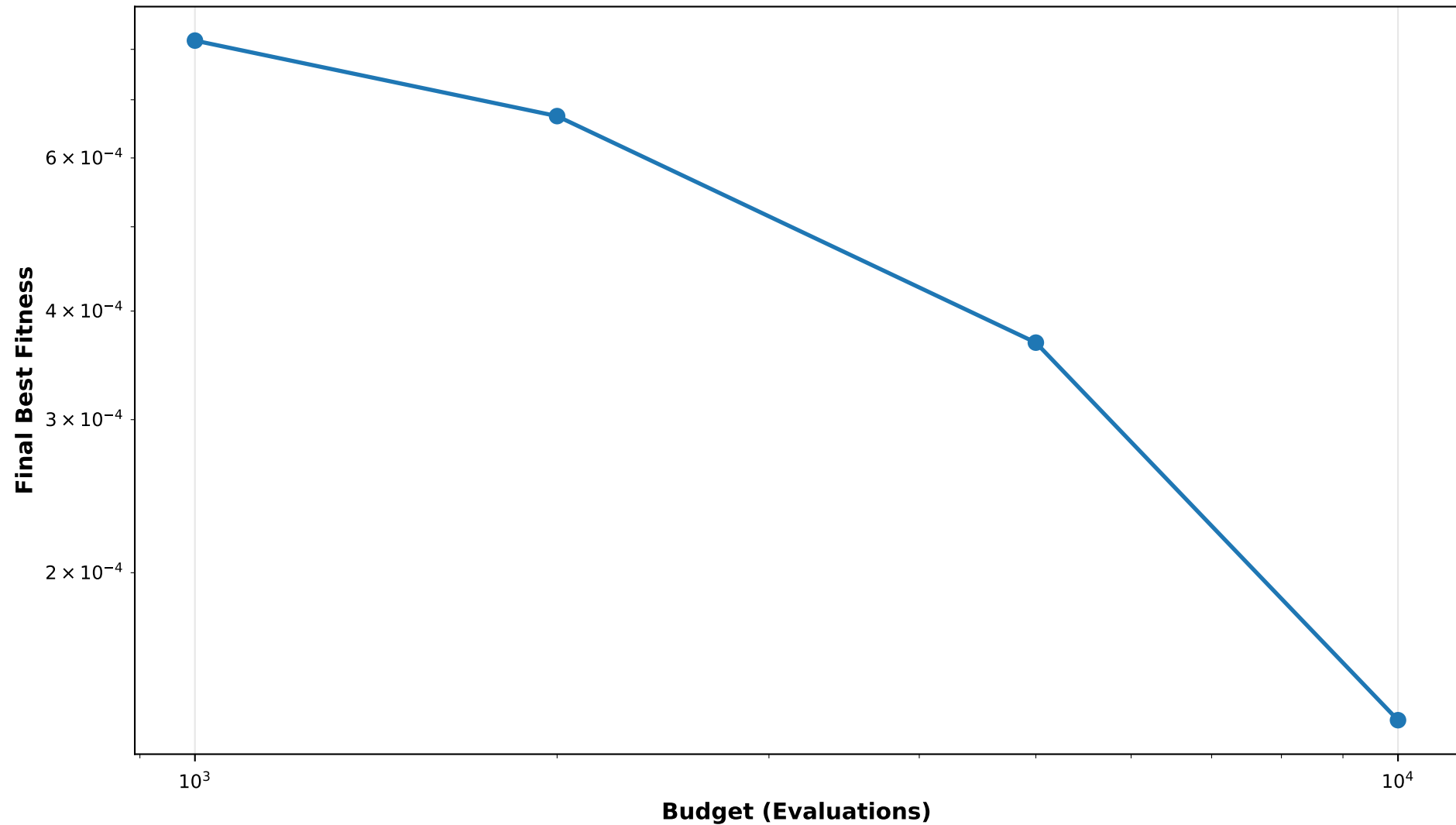
Sample Efficiency
