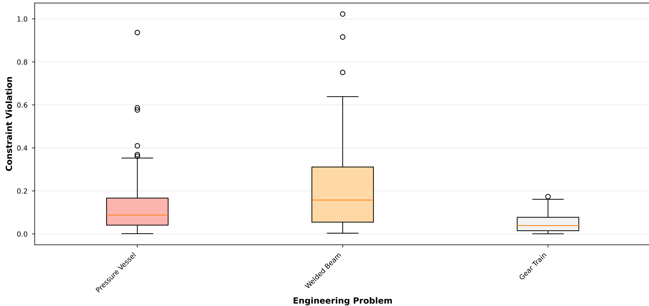
Constraint Violation Distribution
