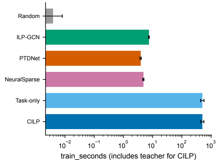
GitHub Developers (CPU)
