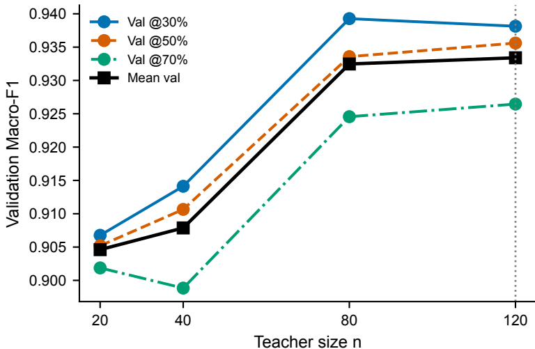
Facebook seed 0 teacher-size sensitivity
