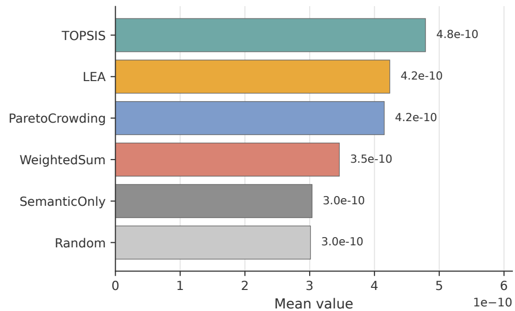
Hypervolume proxy
