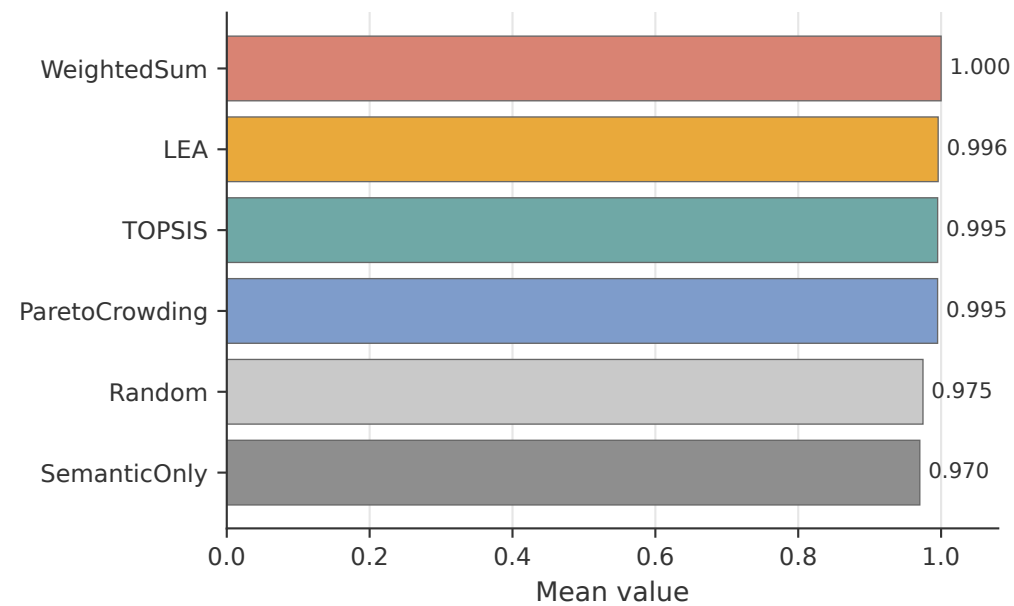
NDCG@K
