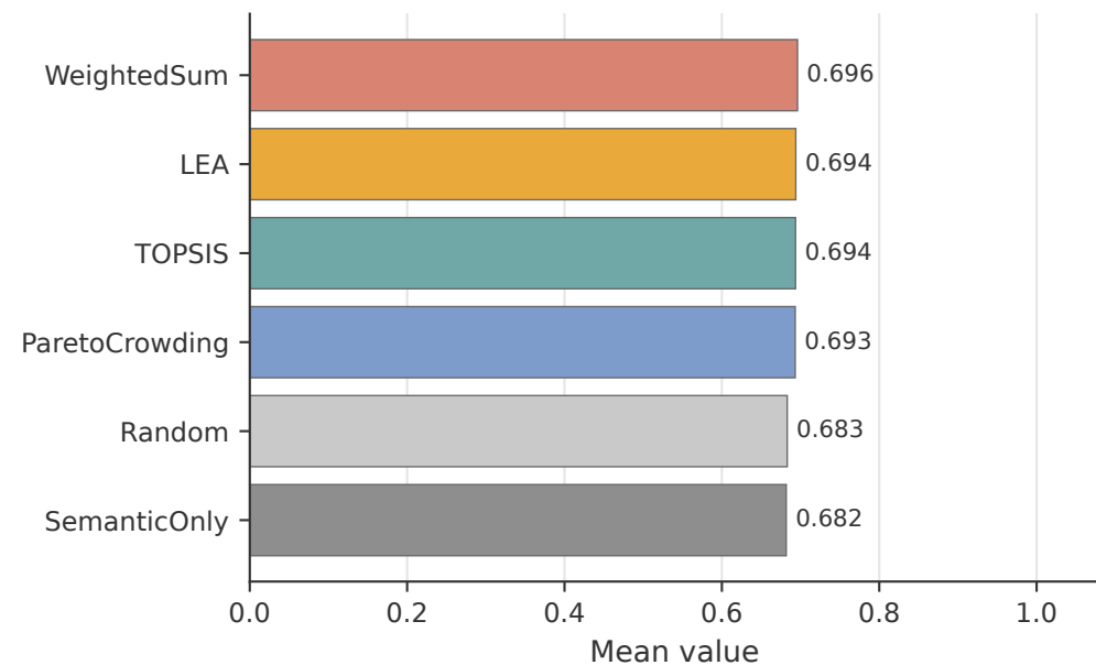
Rel@K
