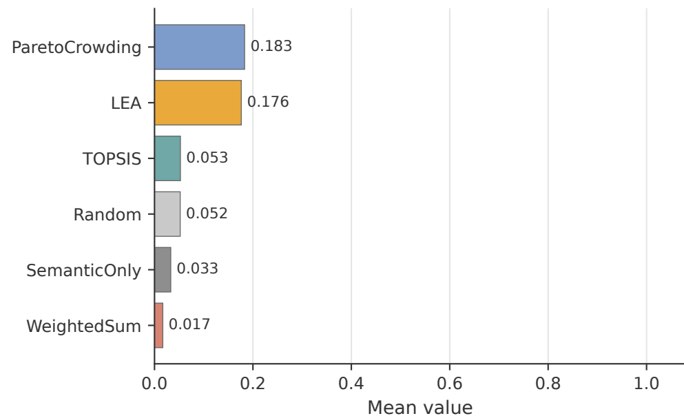
Diversity
