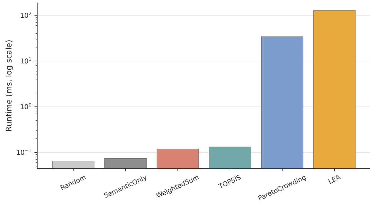
Average Runtime by Ranking Method
