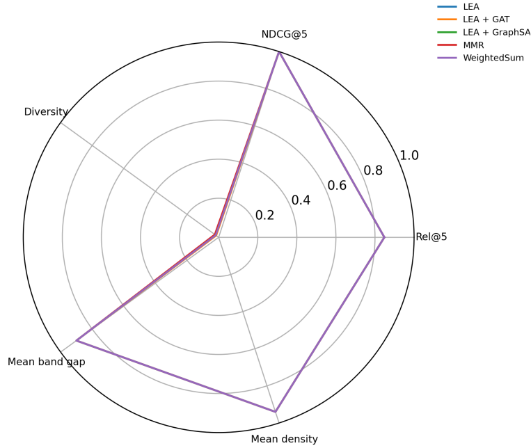
Figure 7: Aggregate method radar profiles comparing WeightedSum, MMR, LEA, and graph-aware LEA variants. Values are means over the evaluated query/seed runs; diversity is a list-level hybrid material distance and the remaining axes are top- K mean objective scores. Void fraction is unavailable for all 20,372 records and is excluded.
