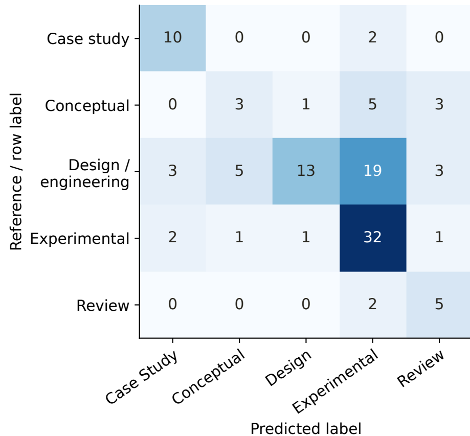
Errors remain concentrated at methodology boundaries
